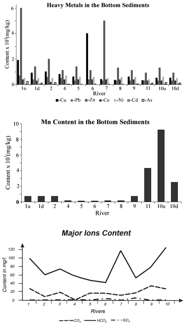
Fig. 4 Heavy metals and manganese contents in the rivers bottom sediments and major ions content in the river water. Rivers: 1-Choroki; 2-Ajaristskali; 3-Bartskana; 4-Korolistskali; 5-Chakvistiskali; 6-Kintrishi; 7-Choloki; 8-Natanebi; 9-Supsa; 10-Rioni; 11-Maltakva (u-upstream, d-downstream)
