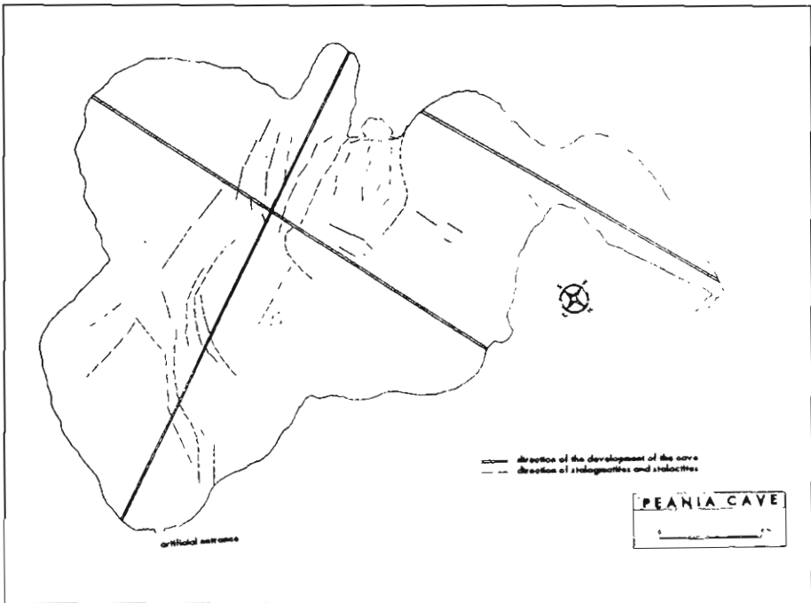
Fig. 4: Plane view of Koutouki cave (Peania, Attica) and the direction of the development of it, in accordance with the main joint sets (after DERMITZAKIS & LEKKAS, 1977).
