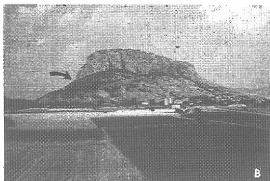
Fig. 1: Photo of the interior of Theopetra cave (A), view of the Theopetra rock mass (B) and schematic cross section (C), after PAPANIKOLAOU & LEKKAS, 1987. 1: Calcareous Cretaceous turbidites, 2: Paleocene red pelites, 3: Tertiary flysch, 4: Ophiolites, 5: Lower Cretaceous Pelagic limestones, 6: Neritic, rudist-bearing limestones, 7: approximated position of the cave.
