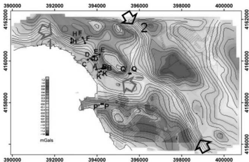
Fig. 2: The residual gravity anomaly map indicates the existence of two possible faults at the investigation area.
