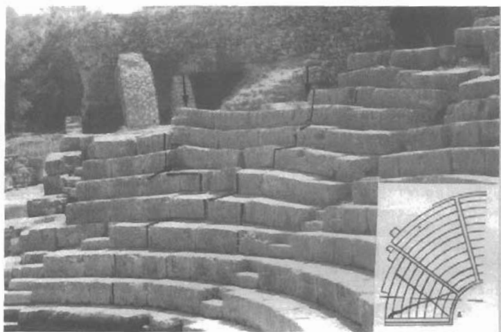
Fig. 6. Photograph of the 3 rd century BC terraced seating (auditorium) of Butrinti Theatre. Deformed construction and especially open fissures are shown by arrows at the western side of the auditorium. Right down corner: the sketch of the diagonal shear cracks.
