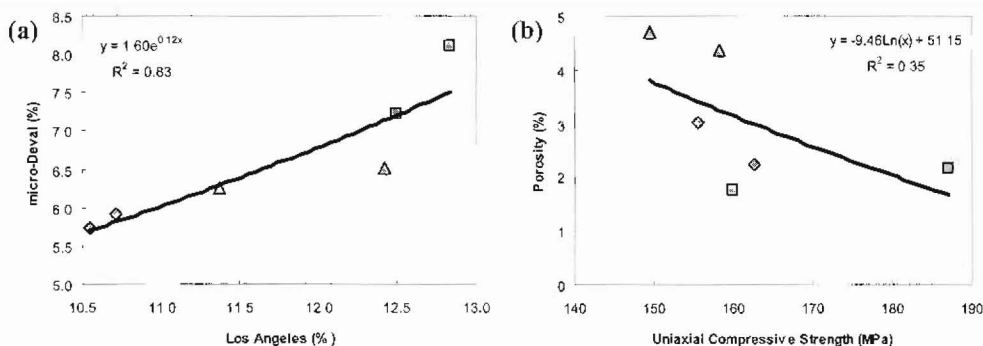
Figure 4 - Relationships between: (a) the micro-Deval and the Los Angeles values, (b) the porosity and the uniaxial compressive strength. Symbols same as in Figure 3
