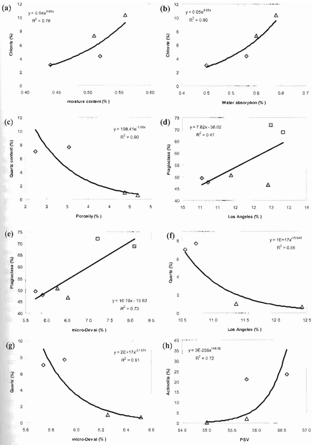
Figure 3 - Relationships between petrographic and physico-mechanical properties: chlorite content plotted against (a) moisture content and (b) water absorption, (c) quartz content plotted against porosity, plagioclase content plotted against (d) Los Angeles and (e) micro-Deval values, quartz content plotted against (f) Los Angeles and (g) micro-Deval values, (h) actinolite content plotted against PSV values (rhombs: group A of dolerites, triangles: group B of dolerites, squares: troctolites)
