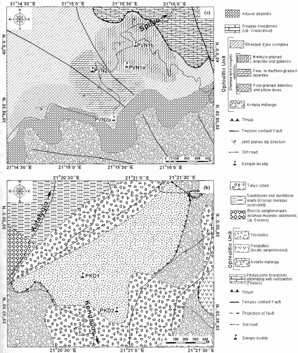
Figure 1 – Geological – sampling map of the a) Spileo and b) Koridallos areas from the Pindos ophiolite complex
