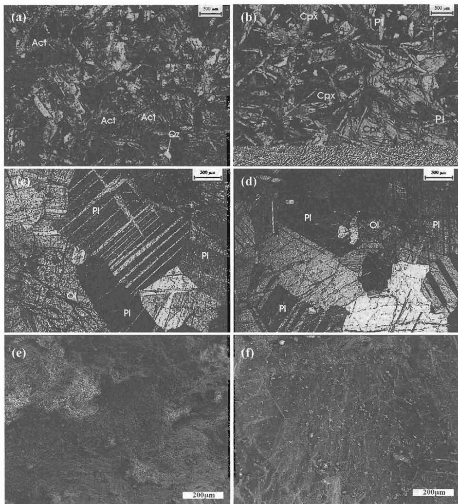
Figure 2 – Polarized photomicrographs of samples a) PVN1a, b) PVN2a, c) PKD1, d) PKD2 (Pl: plagioclase, Ol: olivine, Act: actinolite, Qz: quartz) and Secondary Electron Images showing surface roughness of e) the dolerites (sample PVN1a) and f) troctolites (sample PKD1) from the Pindos ophiolitic complex
