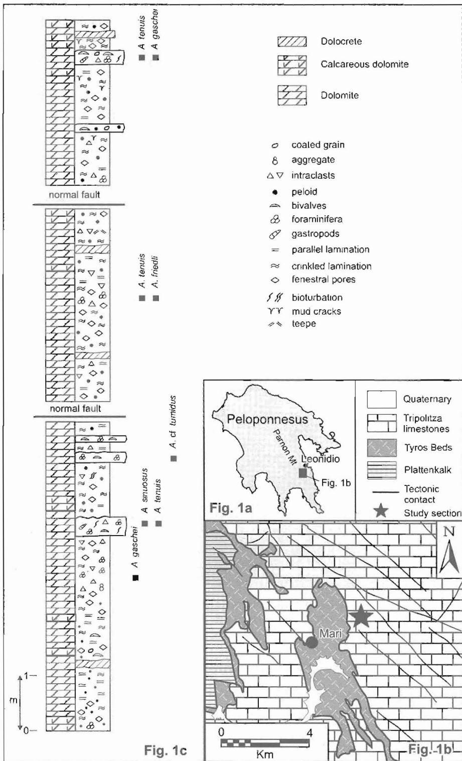
Figure 1 – The study area is situated 2 Km on the northeast of the Mari village, on the eastern flanks of the Parnon Mt. (a, b), Geological map of the study area (b), modified from Skourtsos (2002) (c), Litho-biostratigraphy of the three studied Upper Triassic sections Ψηφιακή Βιβλιοθήκη Θεόφραστος - Τμήμα Γεωλογίας. Α.Π.Θ.
