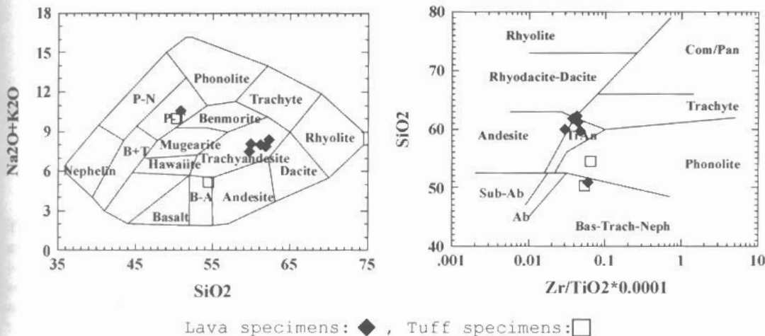
Figure 3. Classification of volcanics according to their alkali (Na 2 O+K 2 O) and silica (SiO 2 ) contents (Cox et.al, 1979) and silica (SiO 2 ) and (Zr/TiO 2 *0.0001) contents (Winchester and Floyd,1977).
