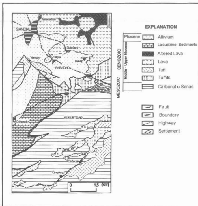
Figure 2. The simplified geological map of the study area
