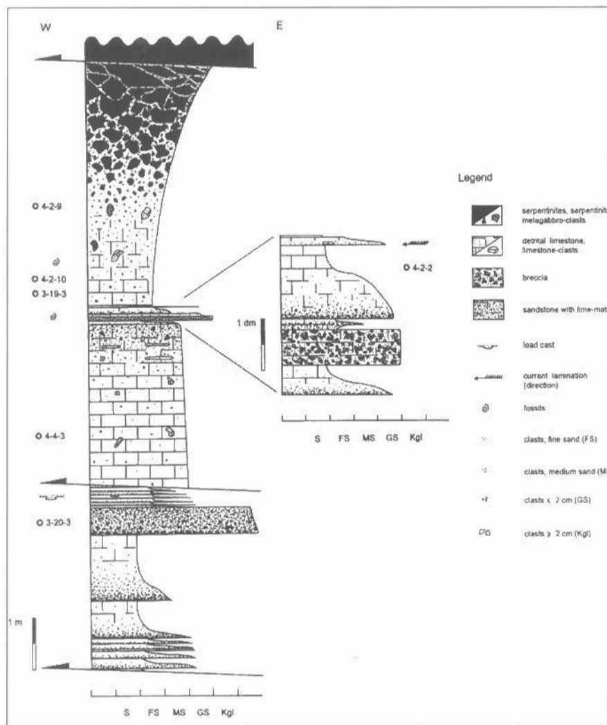
Fig. 2: Stratigraphic type section of flyschoid serpentinite breccias culminating into serpentinitic breccias (see discussion in the text). Road cut at the southern Viglia flank, UTM [x 719940; y 4155070], from Schwandner (1997).
