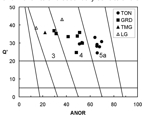
Figure 4. Classification of the analyzed samples of the Brnjica granitoids on the Q-ANOR diagram of Streckeisen & Le Maitre (1979). 3 – granite; 4 – granodiorite; 5a – tonalite.
